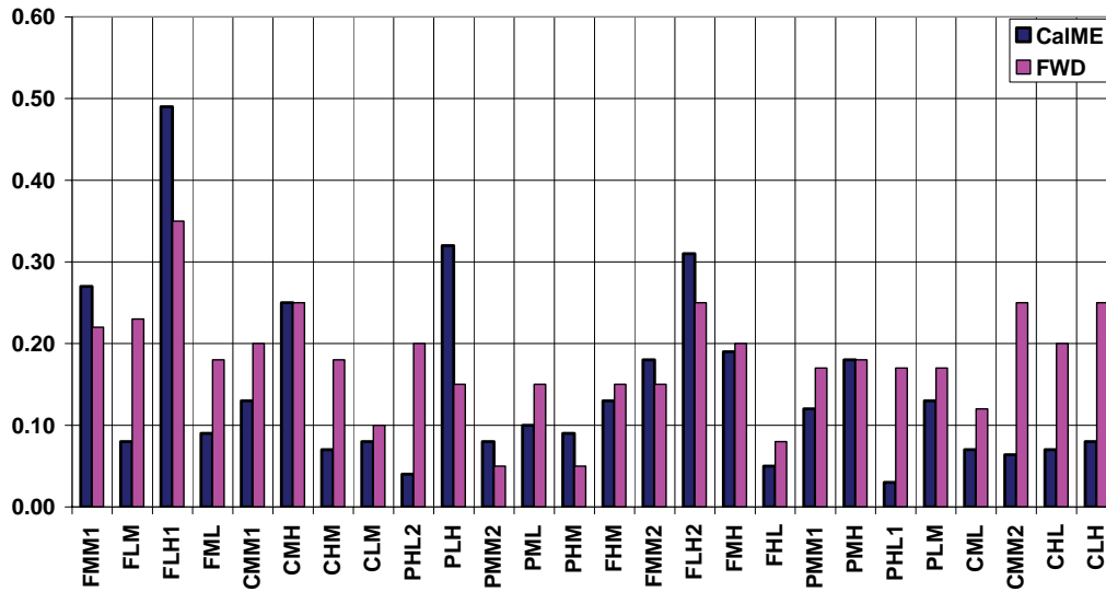
Figure 19. Damage predicted by CalME compared to damage estimated from FWD tests.
