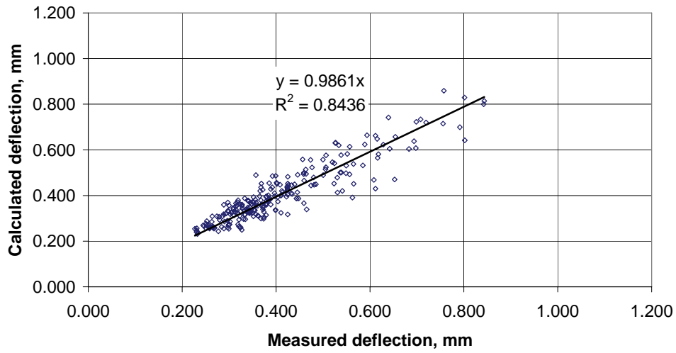
Figure 16. Measured and calculated center deflections on Fine mix sections
