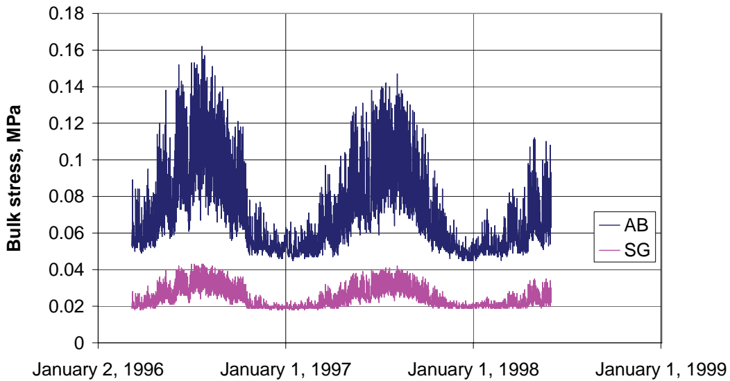
Figure 6. Bulk stress in Aggregate Base and in Subgrade, 50 mm below the surface of the layers, section 18
