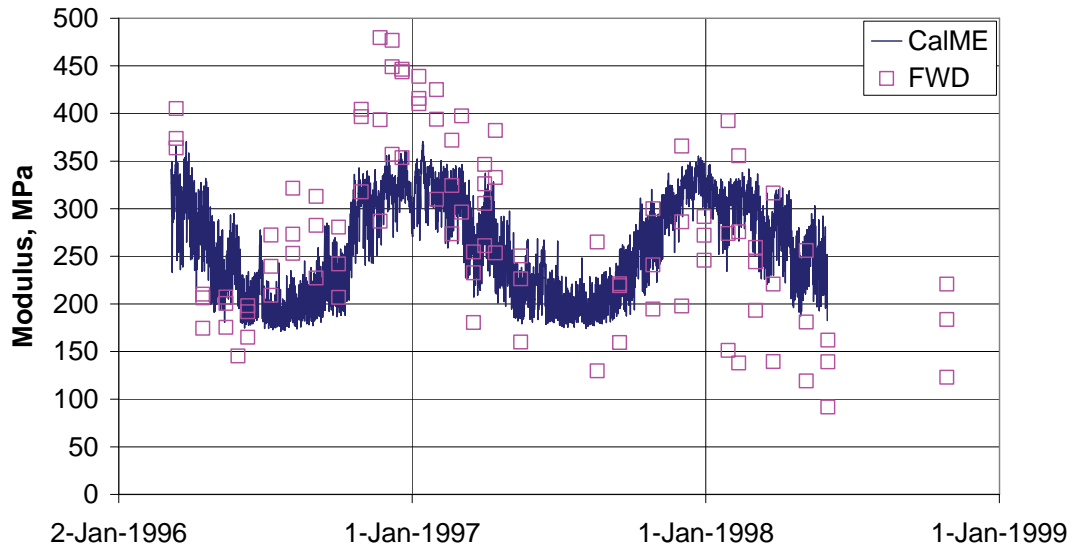
Figure 8 AB moduli calculated by CalME compared to FWD determined moduli.
