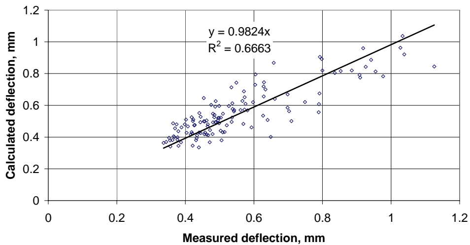
Figure 17. Measured and calculated center deflections on Coarse mix sections.
