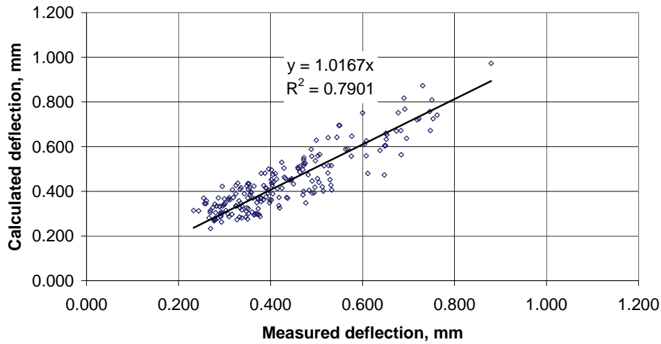
Figure 18. Measured and calculated center deflections on Fine Plus mix sections.
