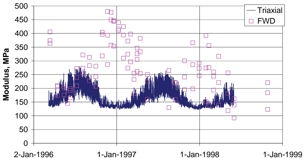
Figure 7 AB moduli at test section 18, from triaxial tests and FWD.
