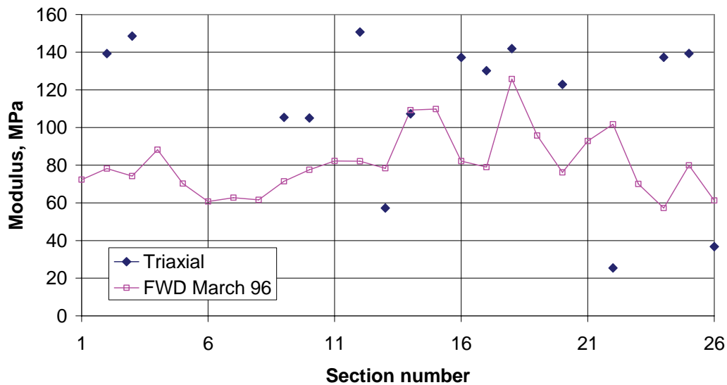
Figure 9. Modulus of Subgrade from triaxial tests and from FWD backcalculation.
